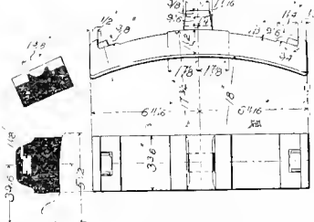
Figs. 4619-4622. BRAKE-SHOE.
